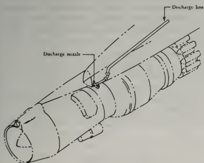
FIGURE 9-15. Fire extinguisher discharge nozzle location.
